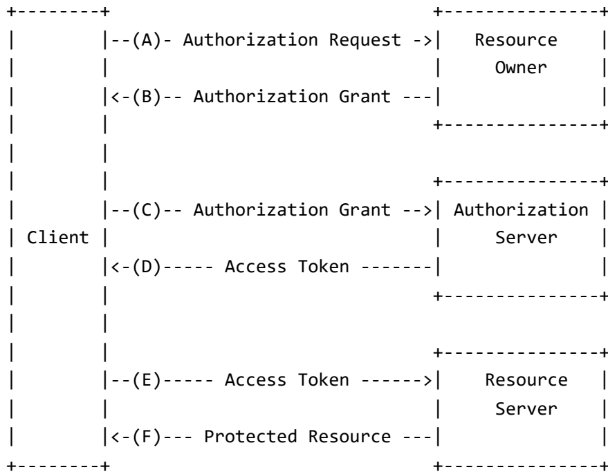
Figure 1: Abstract Protocol Flow
