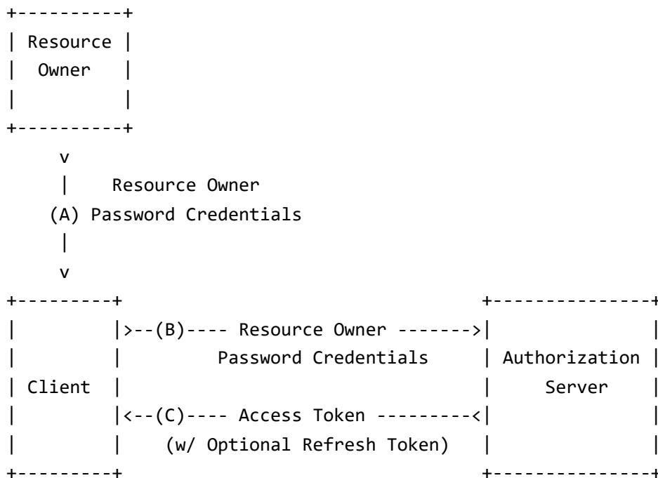
Figure 5: Resource Owner Password Credentials Flow
