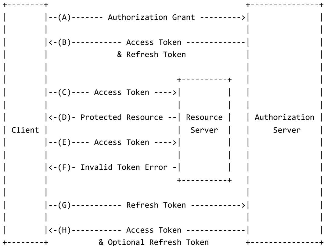
Figure 2: Refreshing an Expired Access Token
