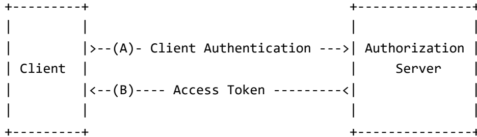
Figure 6: Client Credentials Flow
